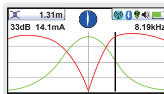
Transverse Graph - displays the field distortion with simultaneous peak and null measurement
