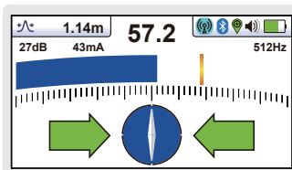
Classic Screen - with on-the-fly colour-coded distortion alert and signal strength bar graph, compass and direction arrows
