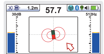
Sonde Locate - 360° arrow guidance to the sonde with distinct symbols and display of depth of cover
