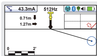
Vector Locate - shows the orientation, line position, and distance of the line in relation to the
