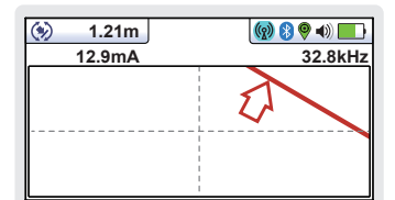
Plan View Screen - displays the theoretical line in 2D from above ground in omnidirectional mode with automatic gain
